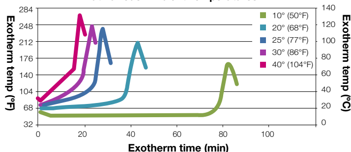
Typical Exotherm Curve for MA422 (10g mass) at Various Ambient Temperatures 5
