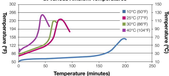
Typical Exotherm Curve for MA530 (30g mass) at Various Ambient Temperatures 5
