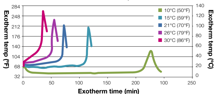
Typical Exotherm Curve for MA550 (30g mass) at Various Ambient Temperatures 5
