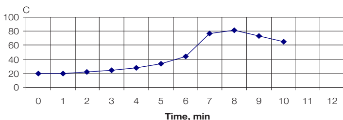
Typical Exotherm Curve for MA3940LH at 23°C (10 grams) 5
