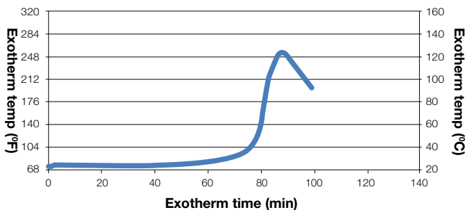
Typical Exotherm Curve for MA2045 (30g mass) 74°F (23°C) 5
