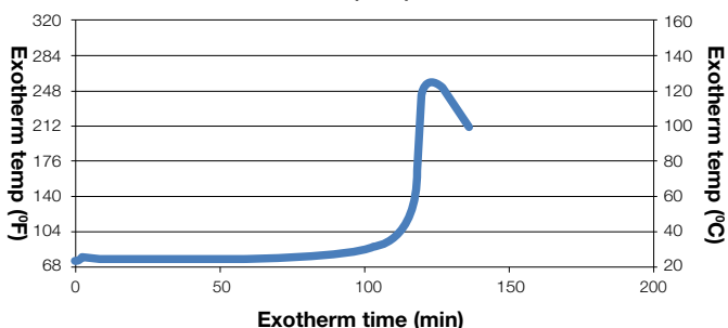
Typical Exotherm Curve for MA2090 (30g mass) 74°F (23°C) 5
