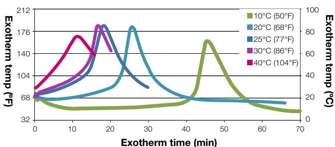
Typical Exotherm Curve for MA3940 (30g mass) at Various Ambient Temperatures 5
