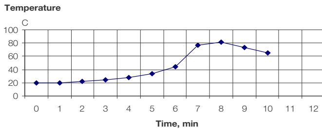
Typical Exotherm Curve for MA3940LH at 23°C (10 grams) 5
