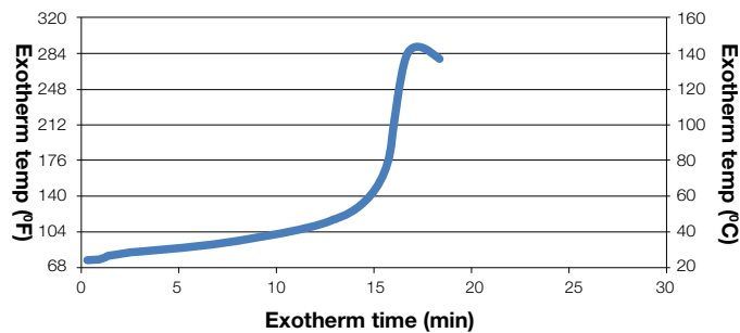
Typical Exotherm Curve for MA8110 (10g mass) 74°F (23°C) 5
